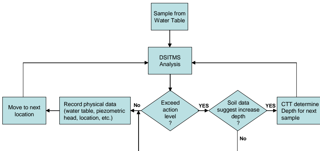
Figure 5. VOC water sampling decision flow chart.
