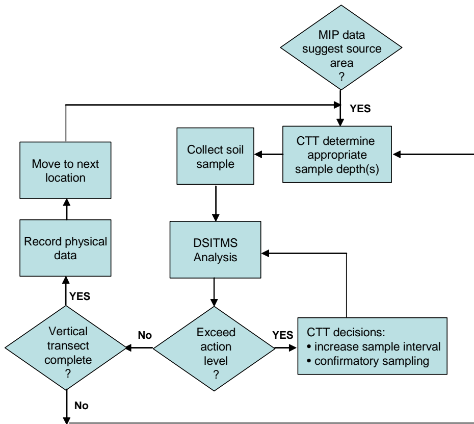
Figure 4. VOC soil sampling decision flow chart.
